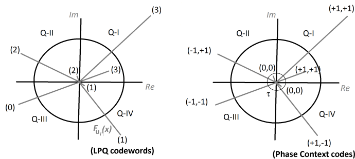
Fig. 1. Local Phase Quantization (left) vs. Phase-Context “no-quantization” (right)
