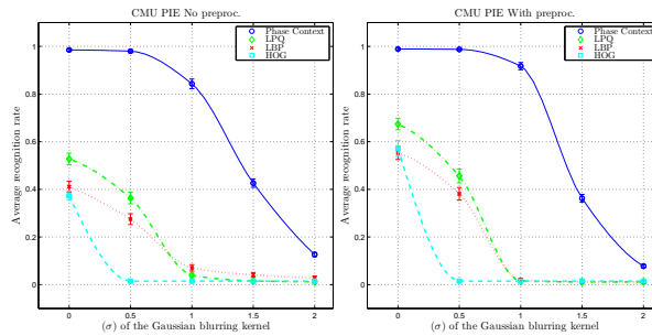
Fig. 6. Average recognition rates on the CMU PIE with increasing blur, No preprocessing (left) vs. with preprocessing (right).
