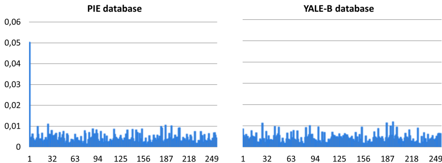
Fig. 4. Comparison of the distribution of code emergence frequency for LPQ codewords (256 codes) on PIE vs. YALE-B database
