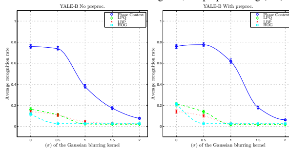
Fig. 7. Average recognition rates on the YALE-B with increasing blur, No preprocessing (left) vs. with preprocessing (right).
