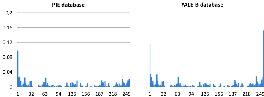
Fig. 3. Comparison of the distribution of code emergence frequency for LBP codewords (256 codes) on PIE vs. YALE-B database
